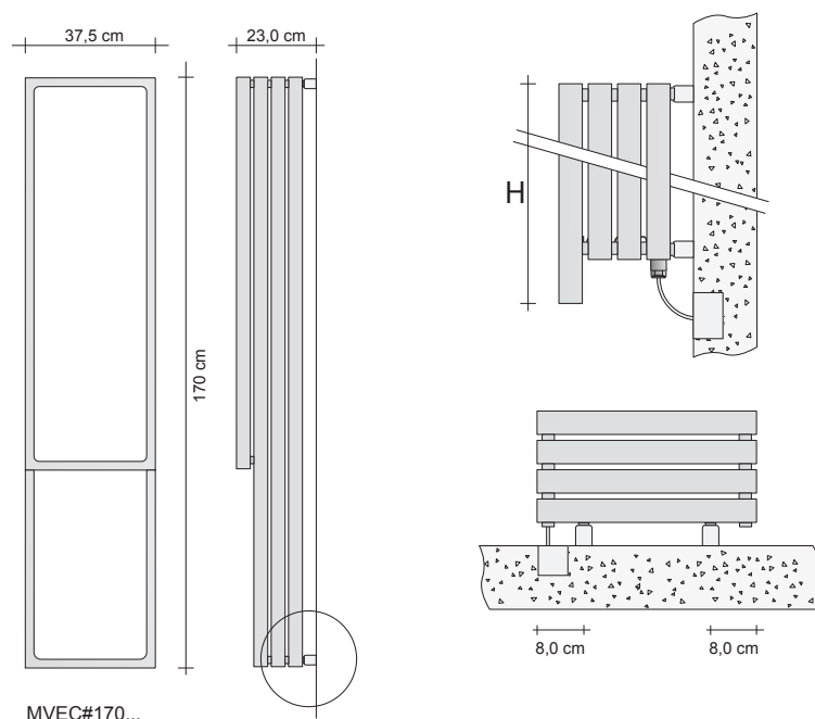
ELECTRIC Connection mod. MVEC#170, MVEC#140 and MQEC#050
