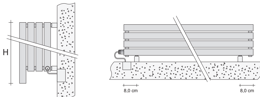
ELECTRIC Connection mod. MOEC#080
